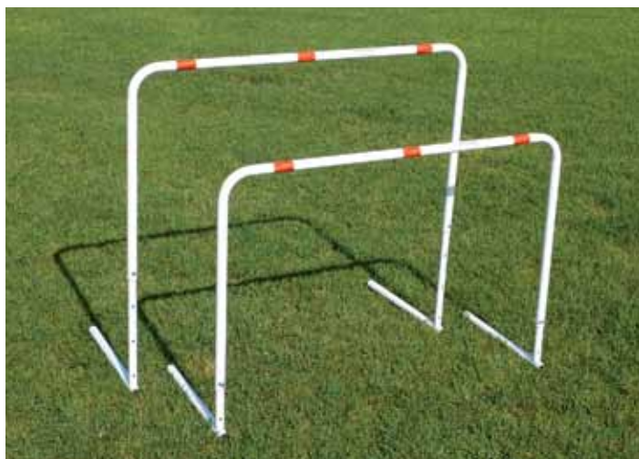
art. 3024 Ostacolo regolabile in acciaio verniciato alt. cm 60-70-80-90 Adjustable hurdle in painted steel, height cm 60-70-80-90
